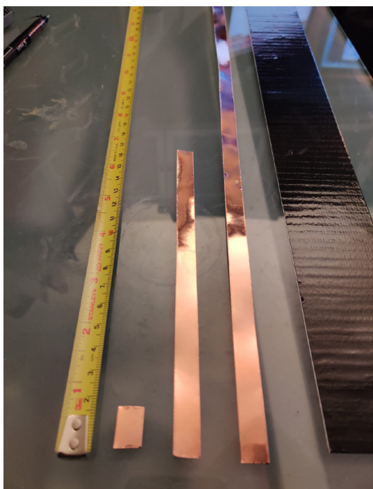
Copper tape preparations for duct tape J-Pole antenna.
