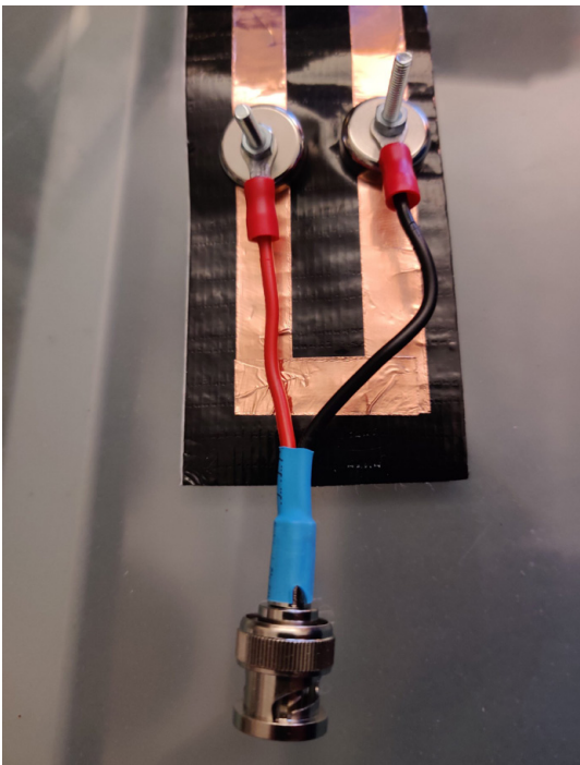
Bestpoke BNC connector to connect a nanoVNA to the copper tape using magnets.
